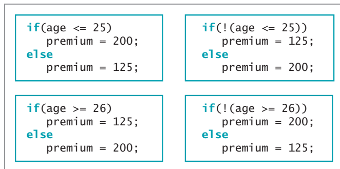
Figure 5-23 Four if...else statements that all do the same thing
