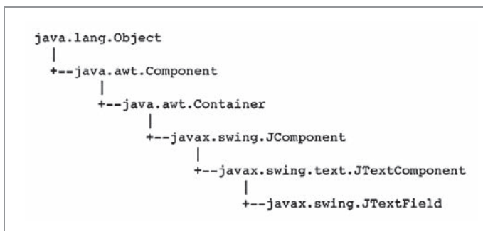
Figure 14-18 The JTextField class inheritance hierarchy
