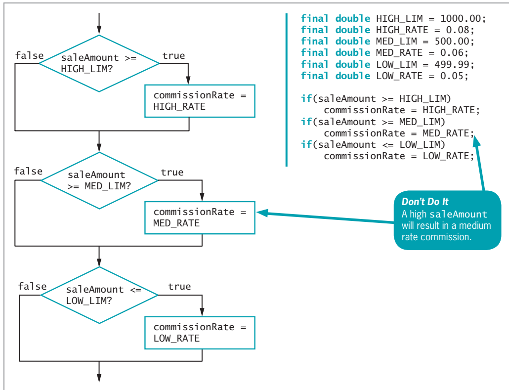
Figure 5-14 Incorrect commission-determining code
