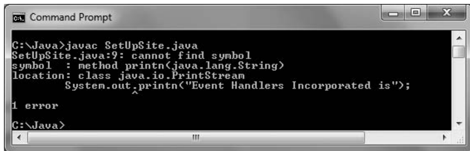
Figure 3-27 Error message received when println is incorrectly spelled
