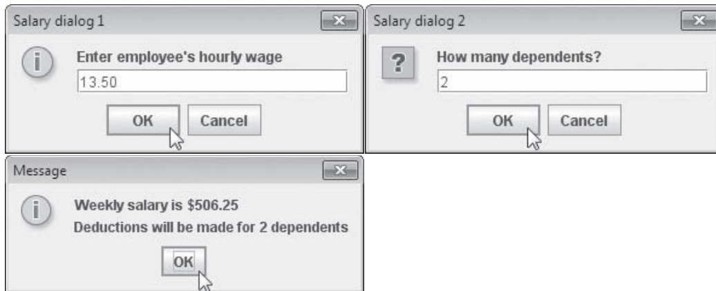
Figure 2-21 Sample execution of the SalaryDialog application
