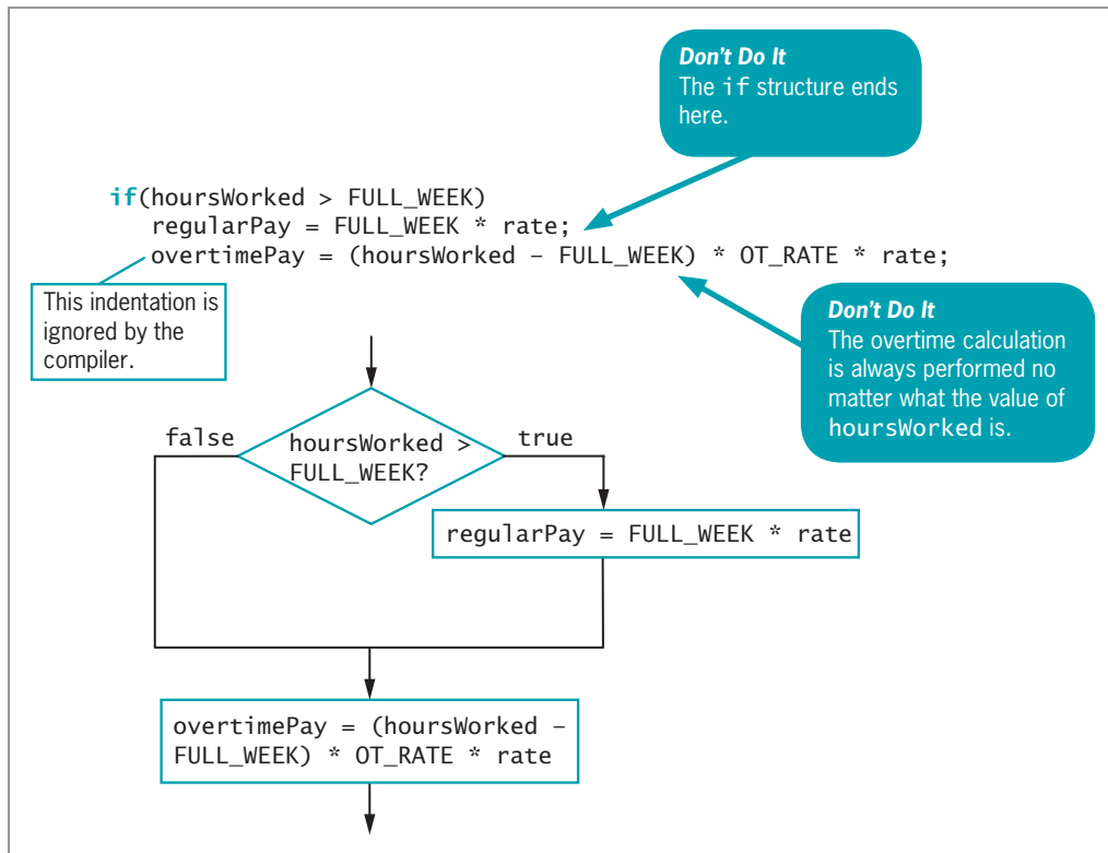
Figure 5-7 Erroneous overtime pay calculation with missing curly braces
