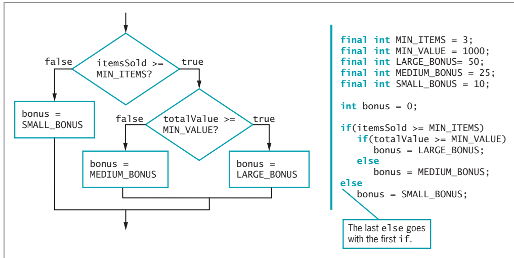
Figure 5-11 Determining one of three bonuses using nested if statements
