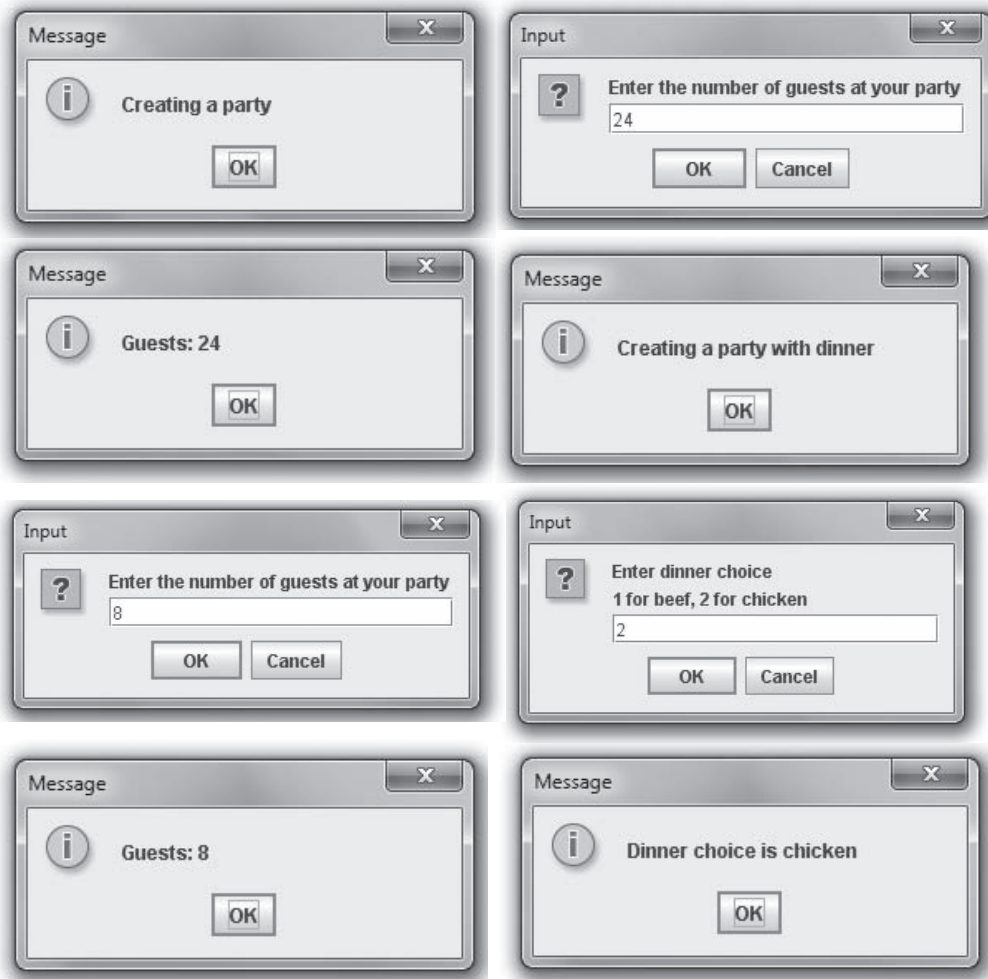
Figure 10-26 Execution of the UseDinnerParty application
