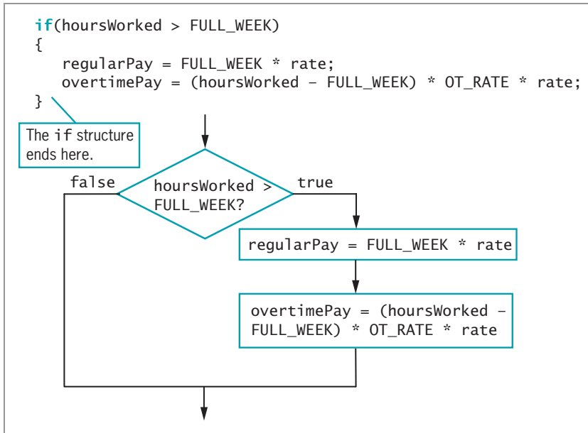
Figure 5-6 An if structure that determines pay
