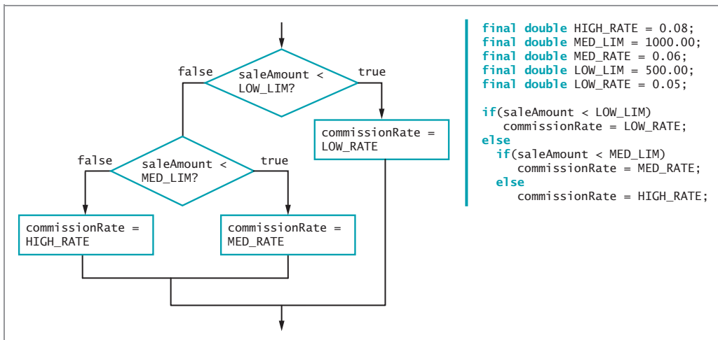
Figure 5-17 Commission-determining code asking about smallest saleAmount first
