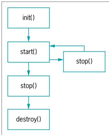
Figure 17-7 The JApplet life cycle
