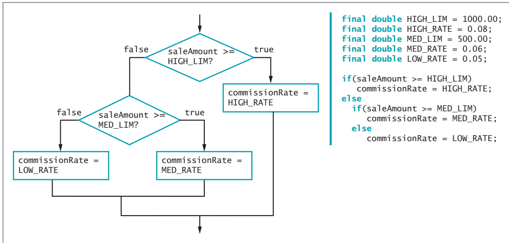
Figure 5-16 Improved and efficient commission-determining logic
