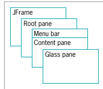
Figure 15-1 Parts of a JFrame
