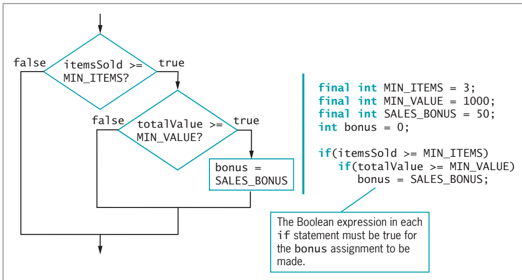
Figure 5-10 Determining whether to assign a bonus using nested if statements
