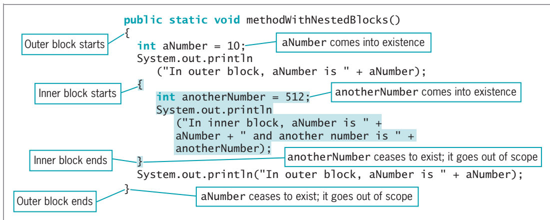
Figure 4-1 A method with nested blocks
