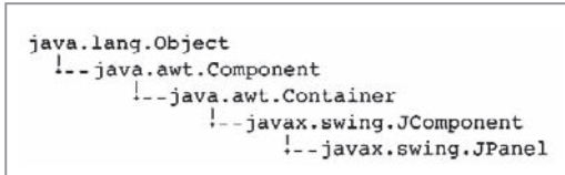
Figure 15-14 The inheritance hierarchy of the JPanel class
