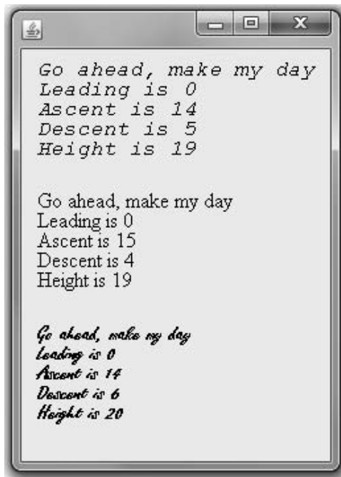
Figure 16-31 Output of the JDemoFontMetrics program
