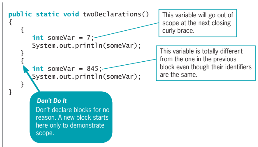
Figure 4-4 The twoDeclarations() method
