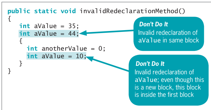
Figure 4-5 The invalidRedeclarationMethod()
