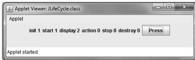
Figure 17-16 The JLifeCycle JApplet when it first executes
