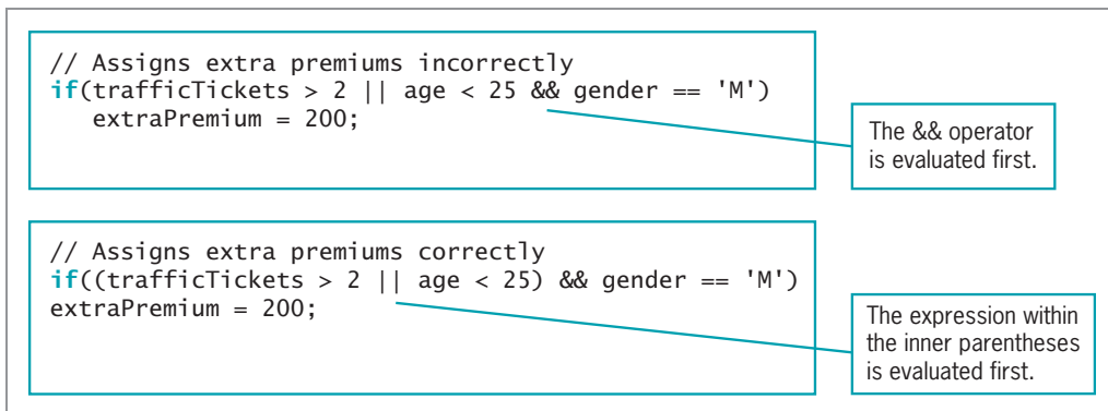
Figure 5-24 Two comparisons using && and ||
