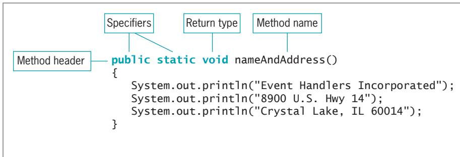
Figure 3-2 The nameAndAddress() method
