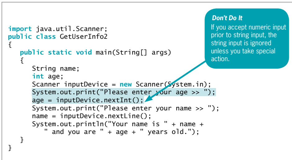
Figure 2-12 The GetUserInfo2 class
