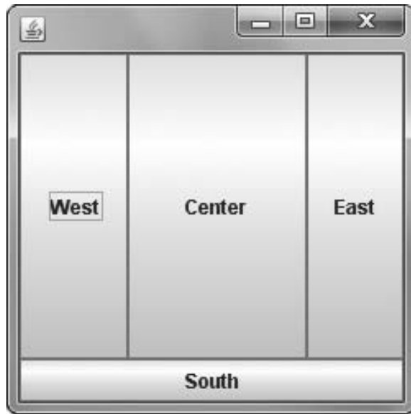
Figure 15-38 Output of the JBorderLayoutNoNorth program
