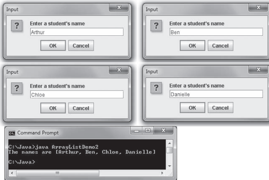
Figure 9-18 Typical execution of the ArrayListDemo2 application
