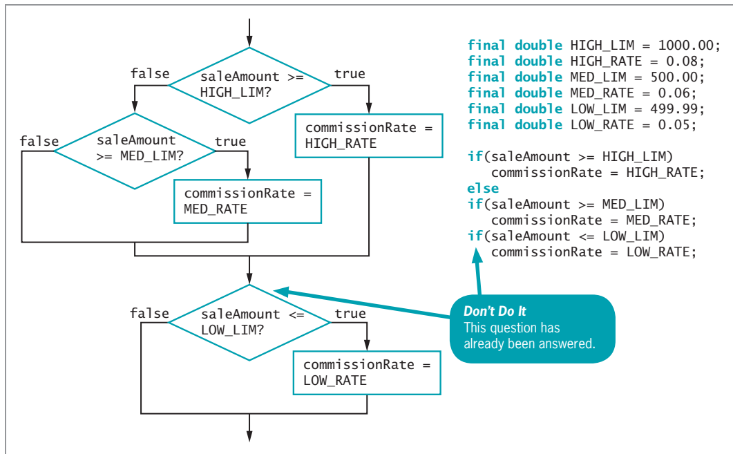
Figure 5-15 Improved, but inefficient, commission-determining code
