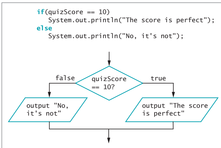
Figure 5-5 An if...else structure
