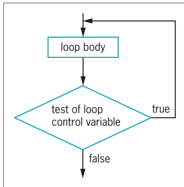
Figure 6-16 General structure of a do...while loop
