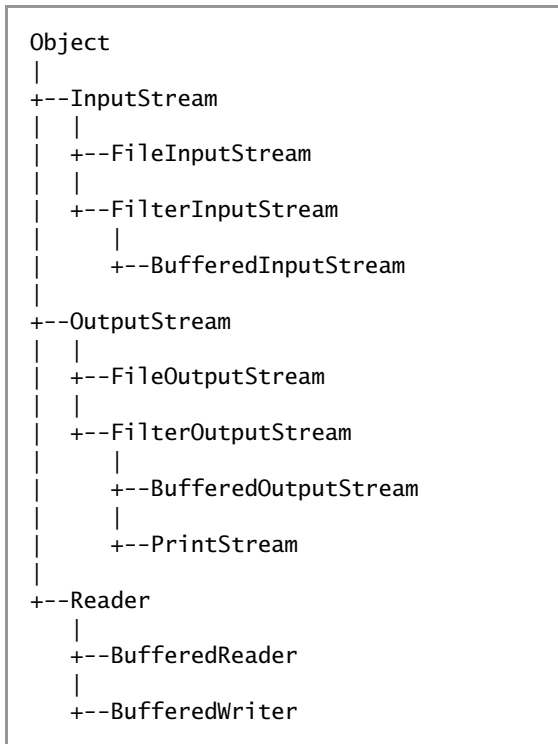
Figure 13-14 Relationship of selected IO classes
