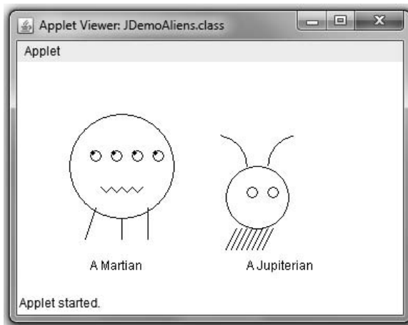
Figure 17-25 Some aliens
