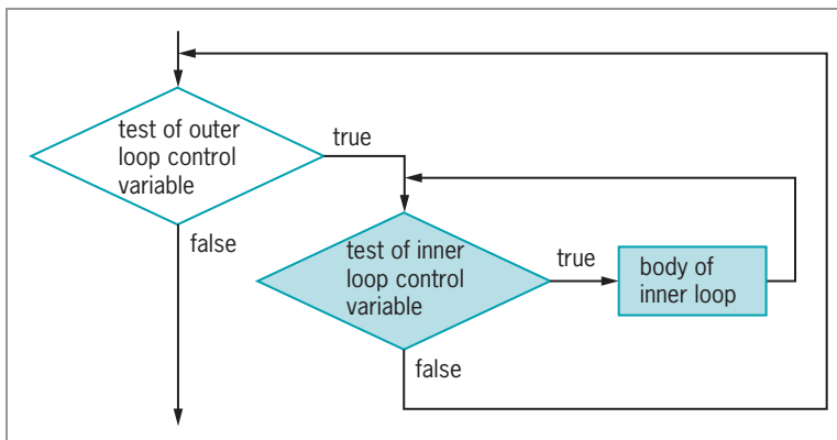
Figure 6-18 Nested loops
