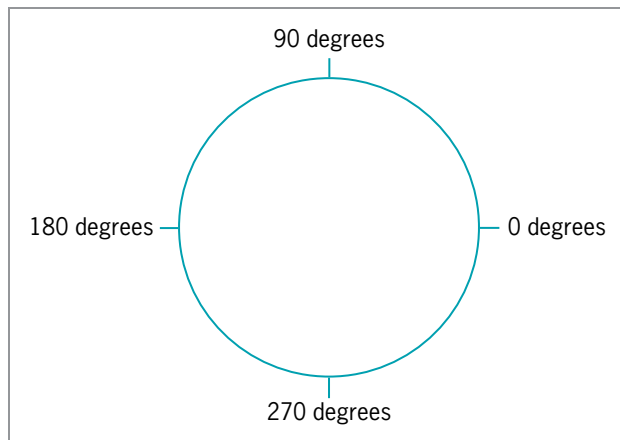
Figure 16-16 Arc positions
