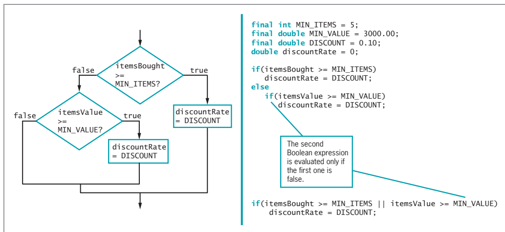
Figure 5-13 Determining customer discount when customer needs to meet only one of two criteria
