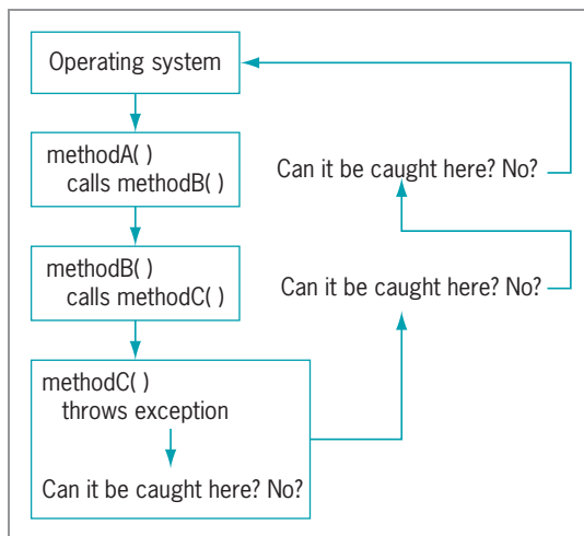
Figure 12-24 Cycling through the call stack
