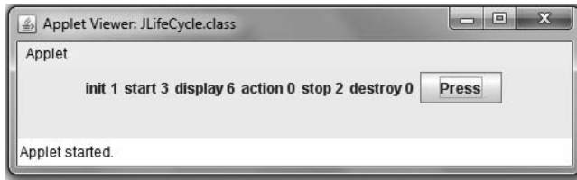
Figure 17-18 The JLifeCycle JApplet after minimizing and restoring twice
