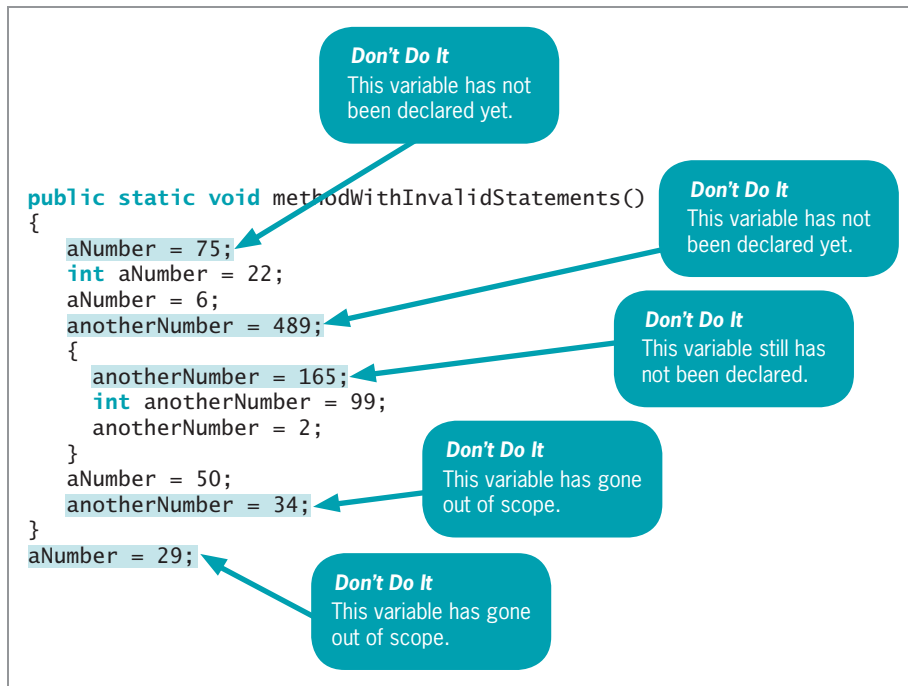
Figure 4-3 The methodWithInvalidStatements() method
