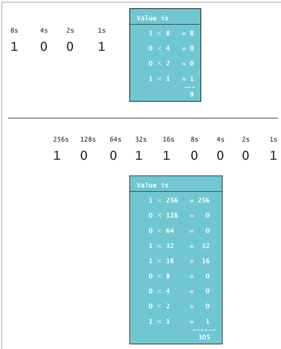
Figure B-2 Representing decimal values 9 and 305 in the binary system
