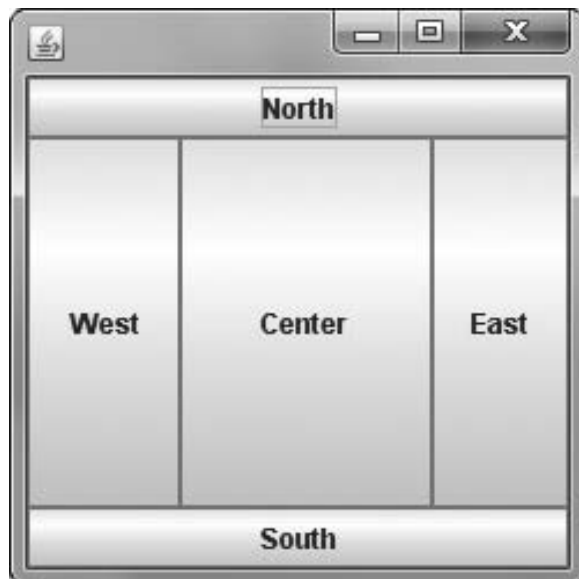
Figure 15-36 Output of the JBorderLayout program
