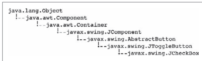
Figure 14-32 The inheritance hierarchy of the JCheckBox class
