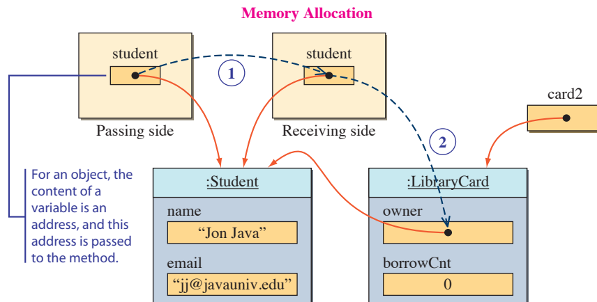
Figure 4.6 This diagram illustrates how an object is passed as an argument to a method.
