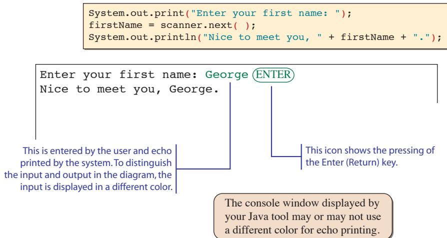
Figure 2.16 Sample interaction using System.in with Scanner and System.out . Keyboard input is echo-printed in the console window.
