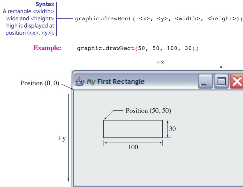
Figure 5.9 The diagram illustrates how the position of the rectangle is determined by the drawRect method.
