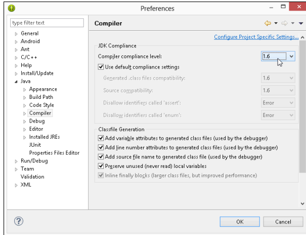
Figure 2-12: Setting the compiler compliance level.
