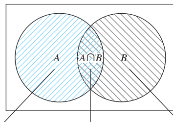
FIGURE 2 The Set of Positive Integers Not Exceeding 1000 Divisible by Either 7 or 11.
