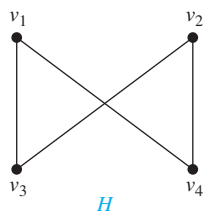
FIGURE 8 The Graphs G and H .
