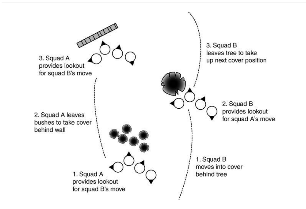
Figure 3.64 Bounding overwatch
