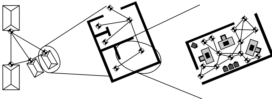
Figure 4.37 Hierarchical nodes
