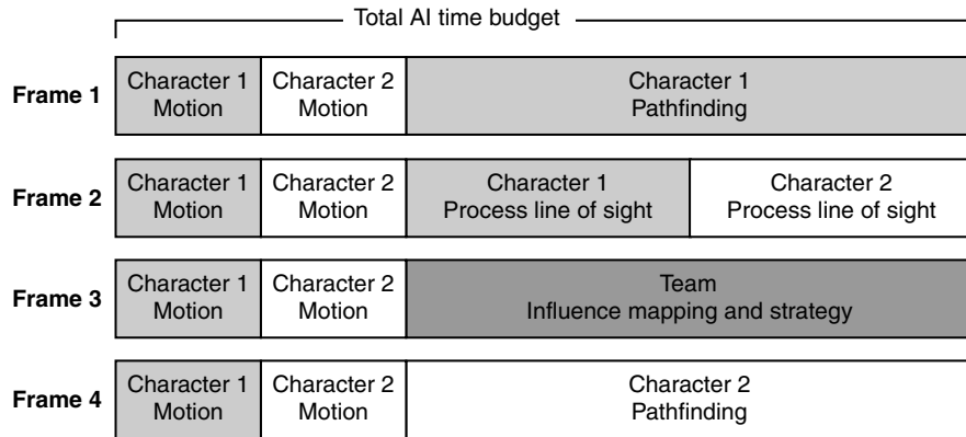
Figure 9.1 AI slicing
