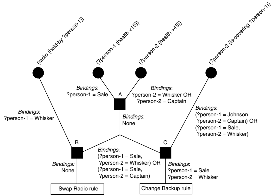
Figure 5.52 Rete after-update
