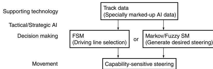
Figure 12.3 AI architecture for race driving
