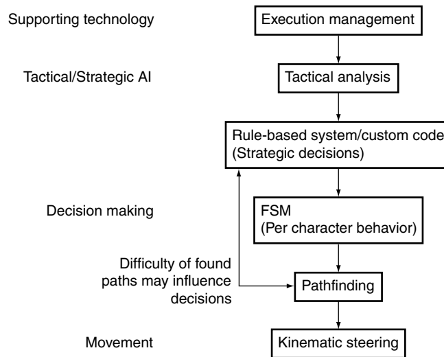
Figure 12.5 AI architecture for RTS games
