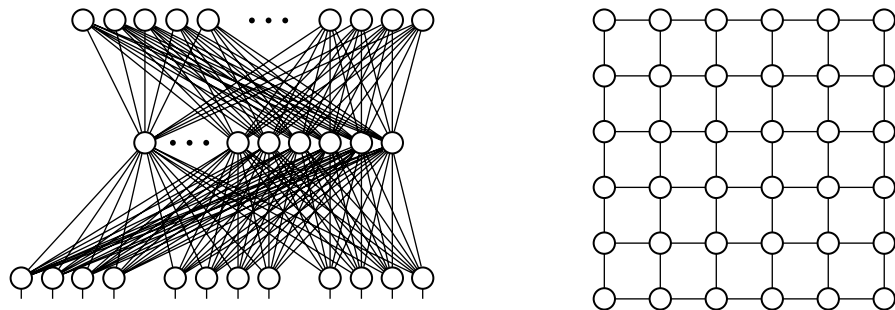
Figure 7.18 ANN architectures (MLP and Hopfield)
