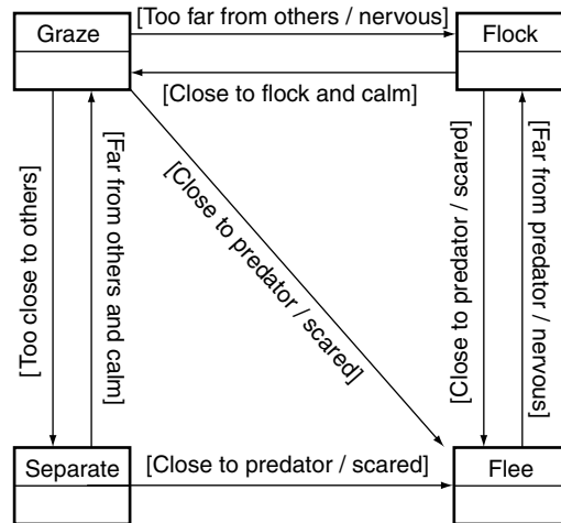
Figure 13.2 A finite state machine for a simple creature
