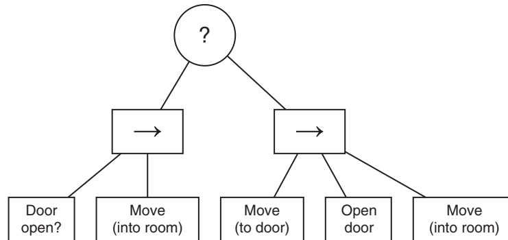
Figure 5.25 A behavior tree with composite nodes
